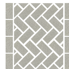
45° Herringbone with header course
